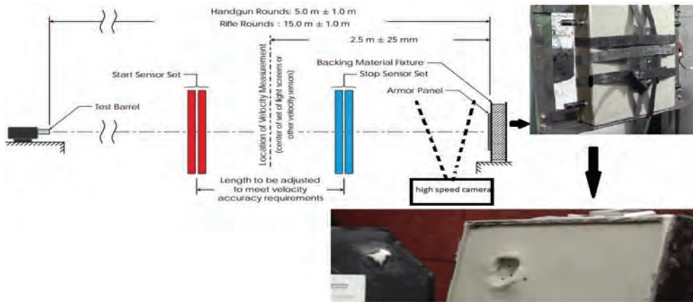
Figure 24. A graphical presentation of a set up for testing the armour panels at the laboratory testing range and images presenting backface deformation (backface signature depth) of a backing material and its response to ballistic impact on the plasticine (or clay) informing about the potential trace in a human body (blunt trauma) that that the fired projectile may cause. Although in an original graphical presentation of a set up presented in the Standard-0101.06 of NIJ, there is no high-speed camera, in many cases, this type of the camera is placed to observe and record the collision of projectiles with a protective panels; source: adapted from graphic [53]; images: top—Oregon Ballistic Laboratory test; bottom—modified on the base of IIIA Soft Body Armor Penetration in Ballistics Clay—AR500 Armor®.
