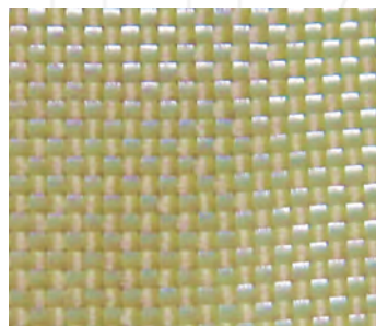
Figure 6. Plain weave fabric made of Kevlar 49® yarns by DuPont; source: author’s own photo archives. Note: Plain weave single fabric; 85 warps/10 cm and 85 wefts/10 cm. Both warps and wefts are made of Kevlar. Total area density: 300 g/m 2 . Thickness: 0.35 mm.
