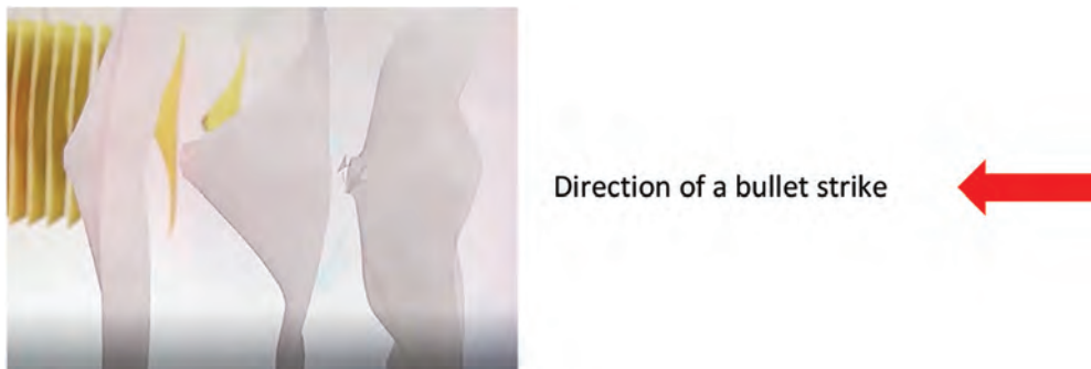
Figure 15. Characteristic cone shapes in the layers of a soft protective panel elements after the bullet struck and perforated them, heading in the direction of the next layer. The cones become smaller due to the smaller amount of bullet kinetic energy transferred to each consecutive layer; prepared on the basis of a Tensylon™ commercial released by DuPont.
