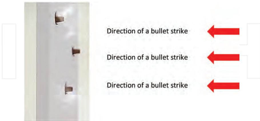
Figure 16. The characteristic indentions in the hard body armour and mushroomed projectiles after they struck the panel and perforated it; prepared on the basis of a Tensylon™ commercial released by DuPont.
